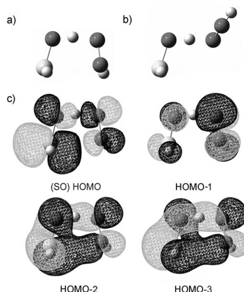
Figure 2. a) Cisoid and b) transoid transition-state structures for the HSOH/OOH reaction. c) The four highest occupied molecular orbitals of the structure in (a) showing the overlap between the sulfenic acid S atom and the internal peroxy O atom.
