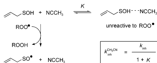
Scheme 1. Mechanistic scheme to explain the observed increase in the rate of alliin-inhibited autoxidation in the presence of acetonitrile.
